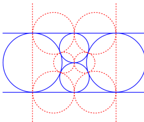
FIGURE 2. Stereographic projection onto \mathbb{R}^2
