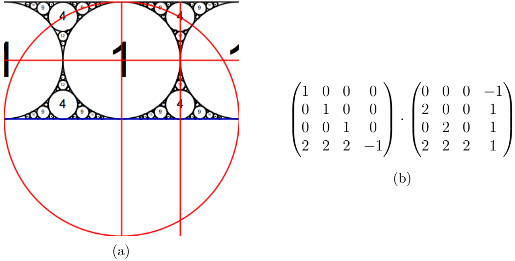
FIGURE 8. (a) Integral packing generated from \widehat{Bi}(1) cluster \{3\} , depicted in blue, along with cocluster, depicted in red. Numbers indicate bends. (b) BV for \widehat{Bi}(1) cluster \{3\} and its orbit, demonstrating integrality of the packing.
