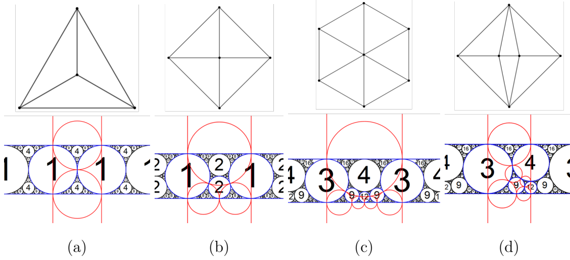
FIGURE 6. (a) Tetrahedron, (b) square pyramid, (c) hexagonal pyramid, and (d) 6v7f 2
