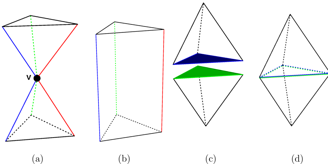
FIGURE 4. Gluing two tetrahedra at vertex \mathbf{v} (a) to produce a triangular prism (b), gluing two tetrahedra along the blue and green faces (c) to produce triangular bipyramid (d)
