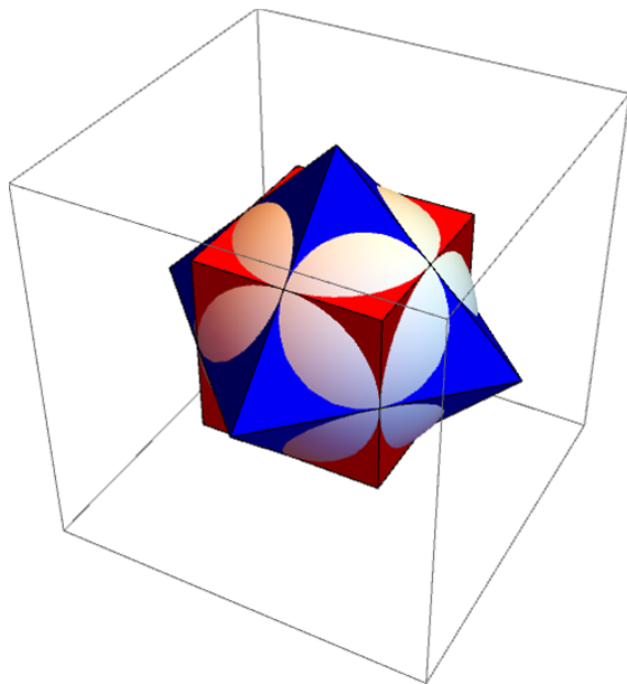
FIGURE 1. Octahedron (blue), its dual (red cube), and midsphere (grey)
