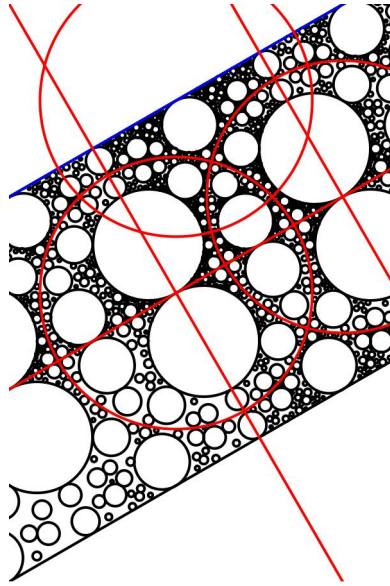
FIGURE 10. A packing arising from cluster \{6\} in §6.2.1.
