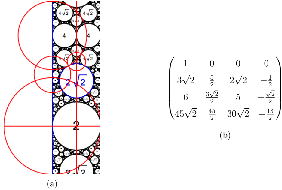
FIGURE 9. (a) Nonintegral packing generated from \widehat{Bi}(14) cluster \{1,8\} , depicted in blue, along with cocluster, depicted in red. Numbers indicate bends. Note mixture of integral and nonintegral bends, indicating that this packing cannot be rescaled to integrality. (b) One of the associated bend matrices B . Note the existence of a nonlinear relation in each row except the first.
