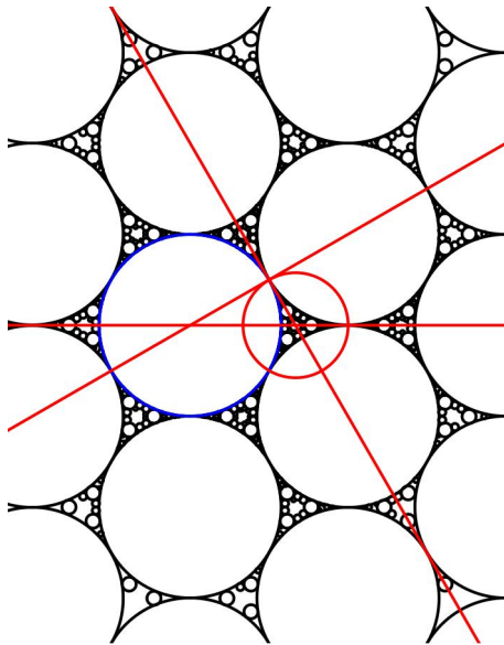
FIGURE 11. A packing arising from cluster \{4\} in §6.2.2.
