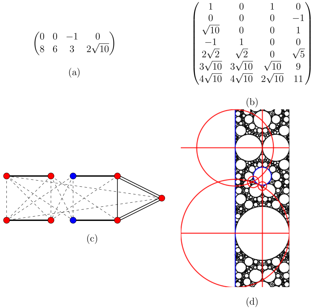
FIGURE 7. (a) Coordinates of cluster \{1,7\} for \widehat{Bi}(10) . (b) Corresponding cocluster coordinates. (c) Coxeter diagram for \widehat{Bi}(10) , with cluster \{1,7\} highlighted in blue. (d) Diagram of \widehat{Bi}(10) cluster \{1,7\} packing, cluster in blue, with cocluster in red.
